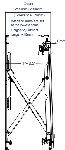
SIDE VIEW OPEN
