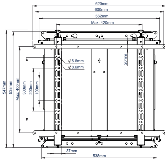
FRONT VIEW WITH ADAPTOR ARMS
