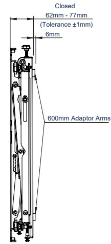
SIDE VIEW CLOSED
